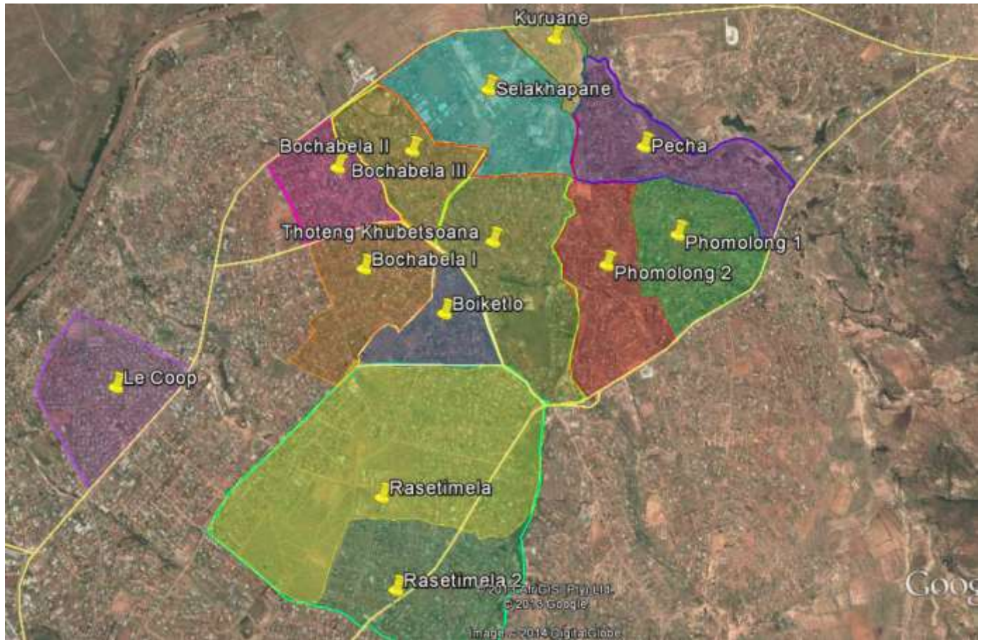
Figure A1. MMC 01—13 clusters (Treatment group)
