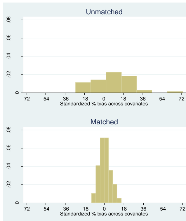
Figure 11. Density distribution of standardize percentage bias across covariates: Comparison of matched and unmatched sample
